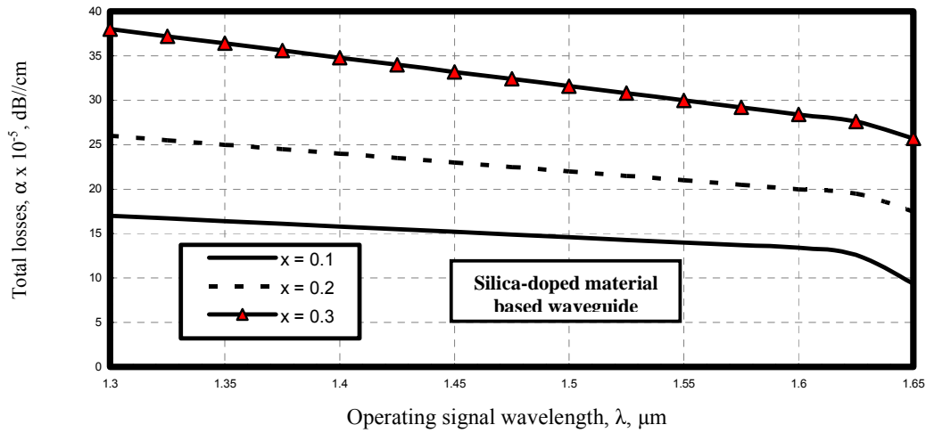
Fig. 12. Variations of total losses against operating wavelength of silica-doped material at the assumed set of parameters.
