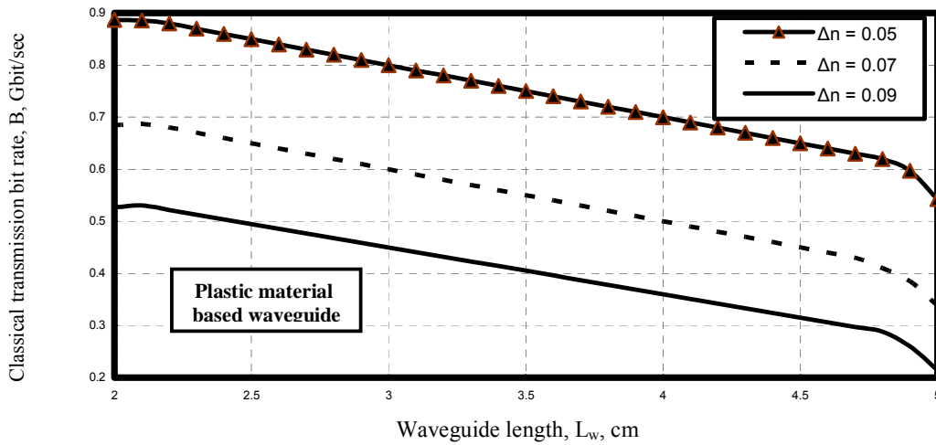
Fig. 15. Variations of classical transmission bit rate versus waveguide length at the assumed set of parameters.
