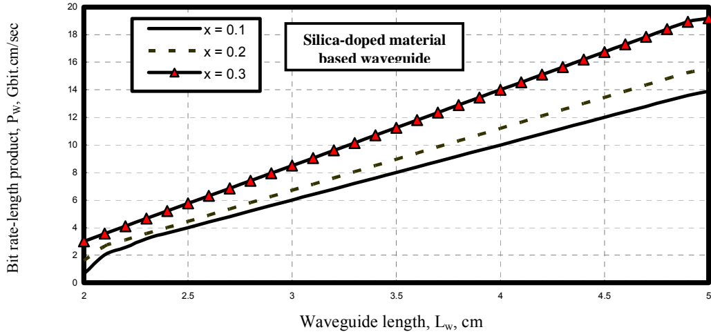
Fig. 17. Variations of bit rate length product versus waveguide length at the assumed set of parameters.
