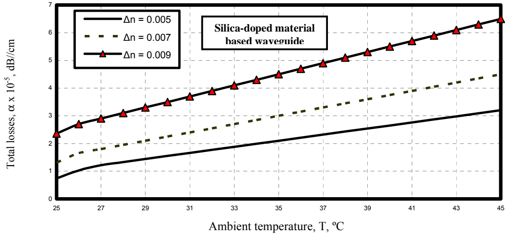
Fig. 11. Variations of total losses against ambient temperature of silica-doped material at the assumed set of parameters.
