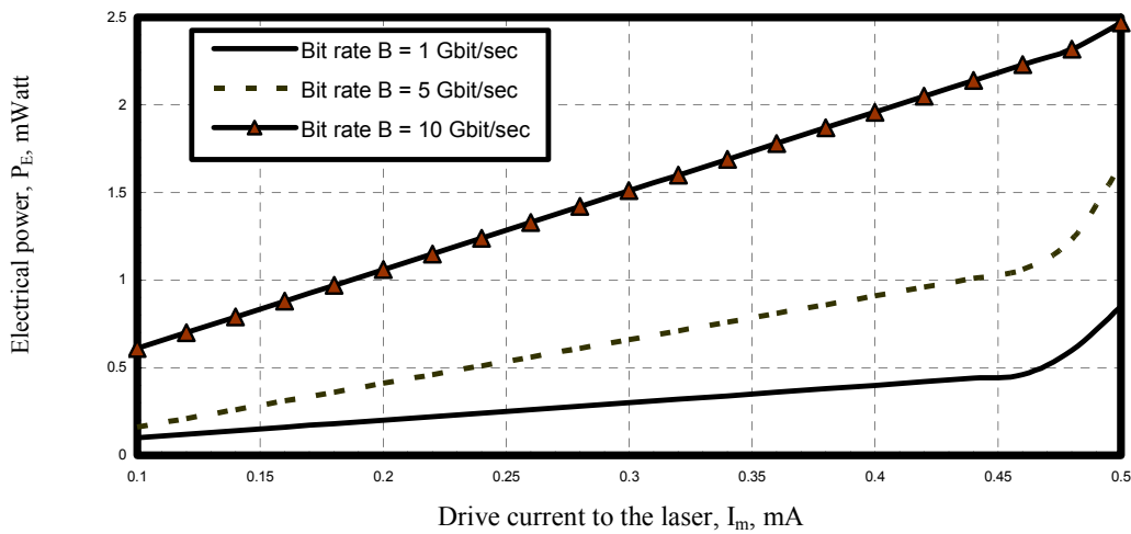
Fig. 3. Variations of electrical power against drive current of the laser at the assumed set of parameters.
