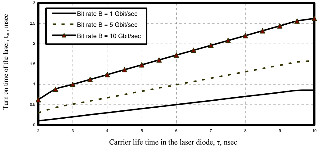
Fig. 5. Variations of turn on time of the laser against carrier life time in the laser at the assumed set of parameters.
