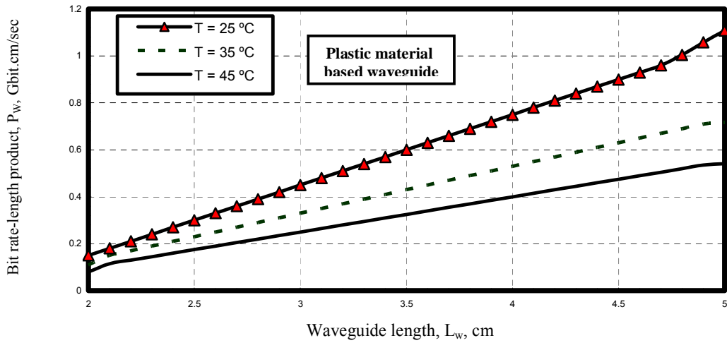
Fig. 18. Variations of bit rate length product versus waveguide length at the assumed set of parameters.
