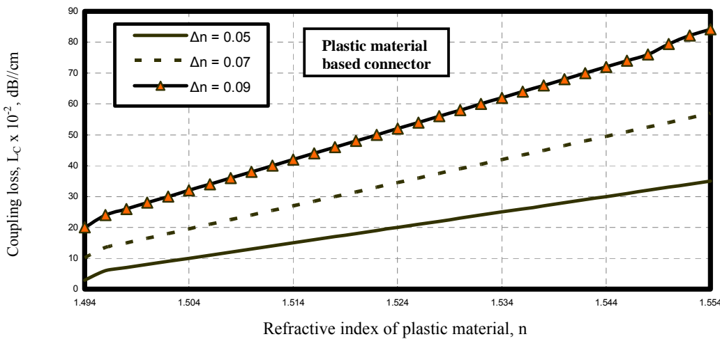
Fig. 10. Variations of coupling loss against refractive index of plastic material at the assumed set of parameters.
