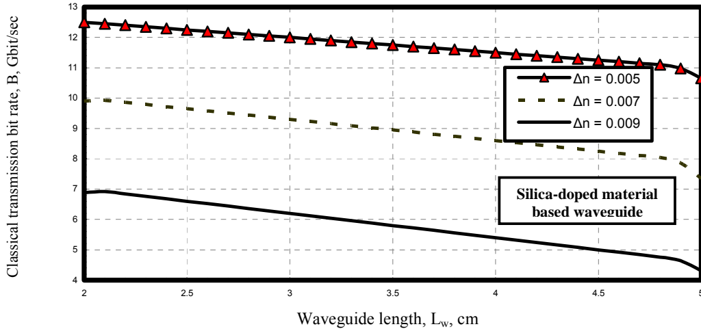
Fig. 14. Variations of classical transmission bit rate versus waveguide length at the assumed set of parameters.
