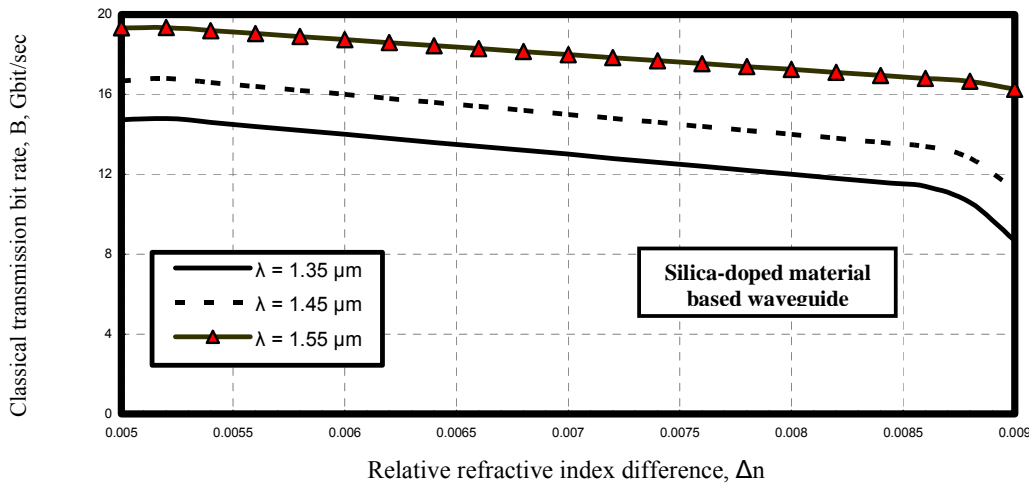
Fig. 19. Variations of classical transmission versus relative refractive index difference at the assumed set of parameters.
