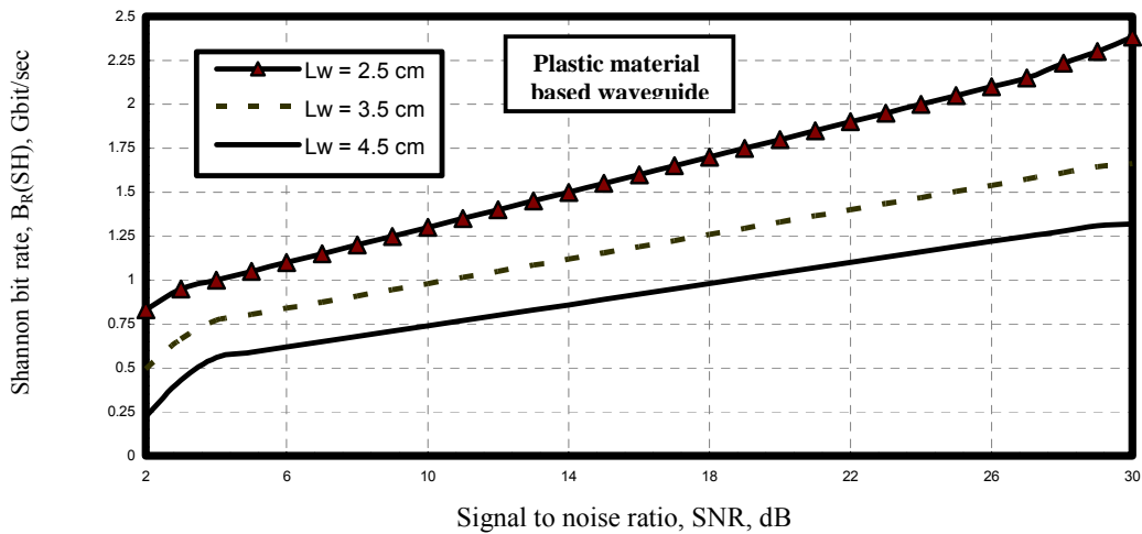
Fig. 25. Variations of Shannon transmission bit rate versus signal to noise ratio at the assumed set of parameters.
