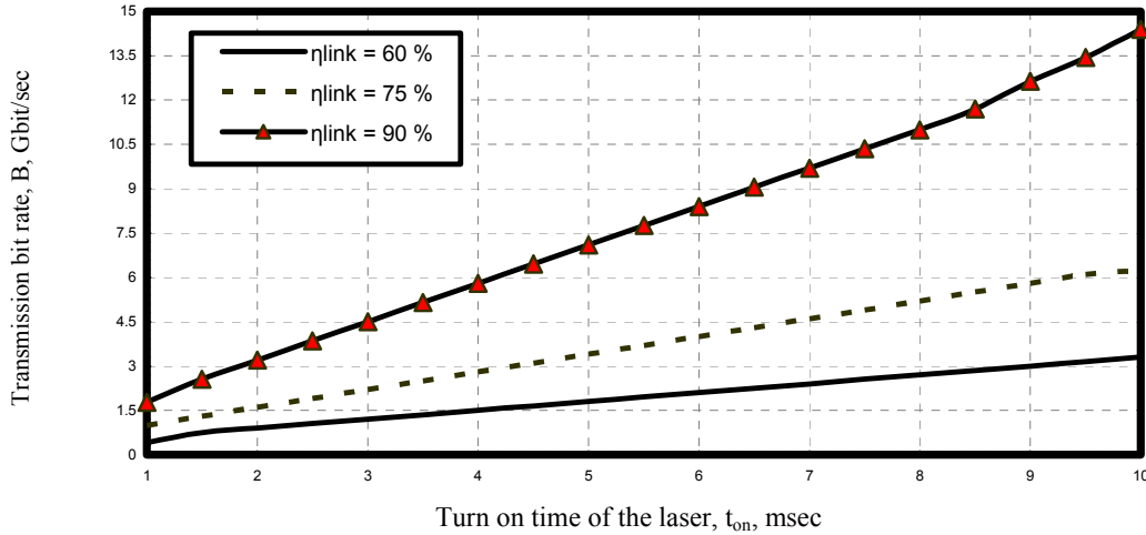
Fig. 8. Variations of transmission bit rate against turn on time of the laser at the assumed set of parameters.
