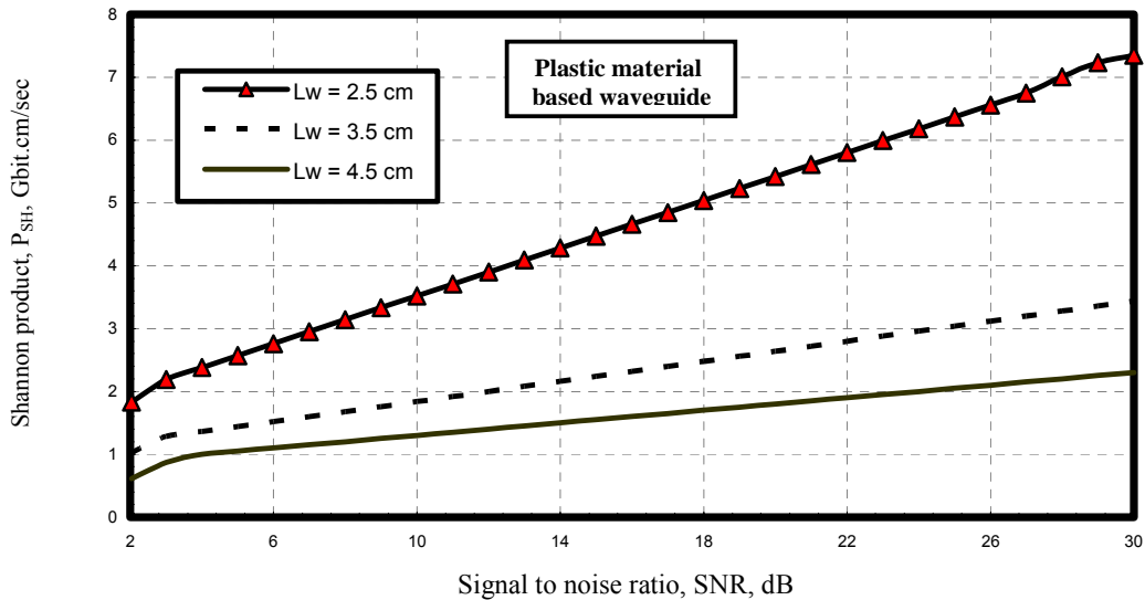
Fig. 27. Variations of Shannon transmission bit rate versus signal to noise ratio at the assumed set of parameters.
