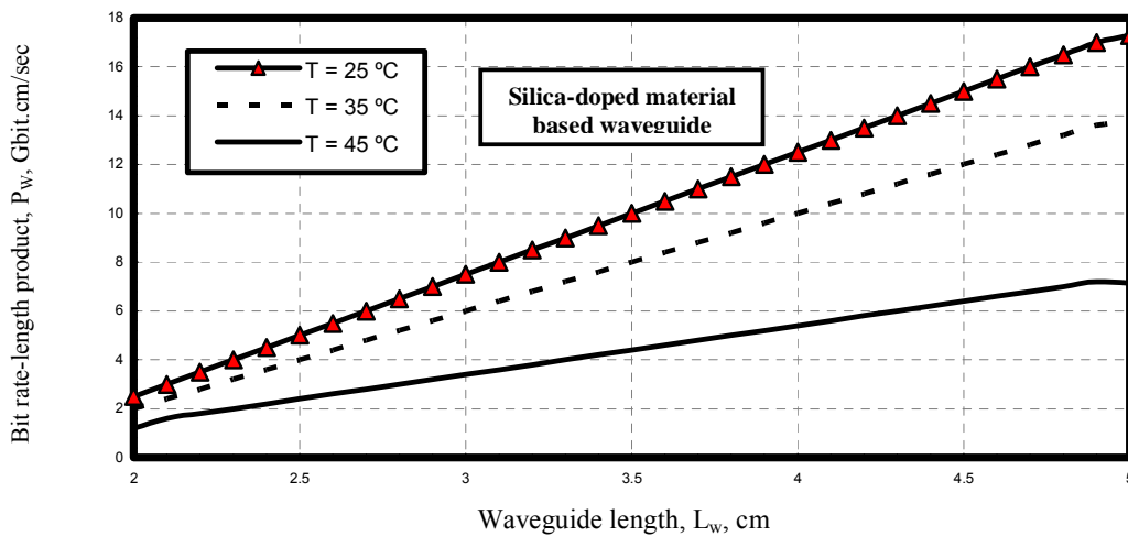
Fig. 16. Variations of bit rate length product versus waveguide length at the assumed set of parameters.
