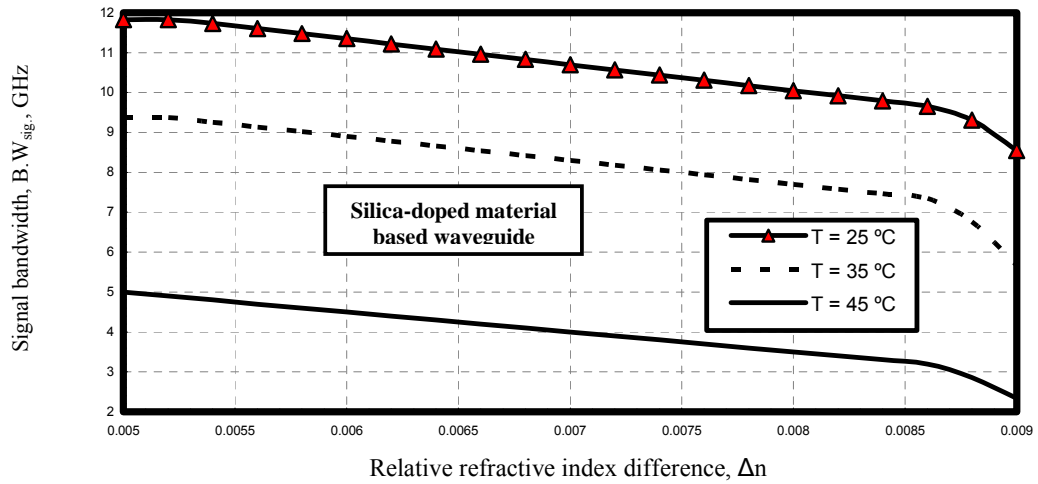
Fig. 21. Variations of signal bandwidth versus relative refractive index difference at the assumed set of parameters.
