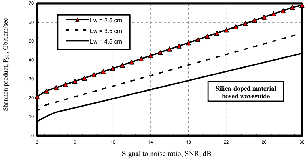
Fig. 26. Variations of Shannon transmission bit rate versus signal to noise ratio at the assumed set of parameters.
