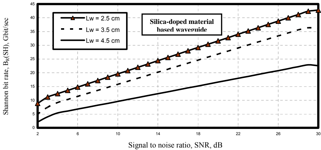
Fig. 24. Variations of Shannon transmission bit rate versus signal to noise ratio at the assumed set of parameters.
