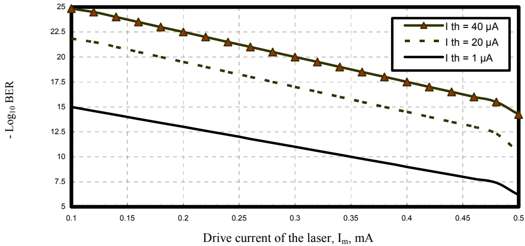
Fig. 2. Variations of bit error rate (BER) against drive current of the laser at the assumed set of parameters.
