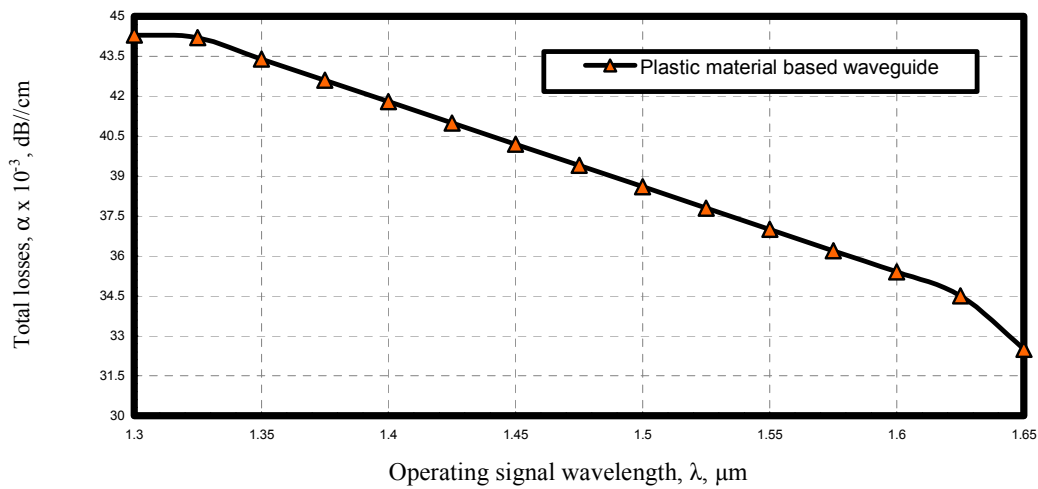
Fig. 13. Variations of total losses against operating wavelength of plastic material at the assumed set of parameters.
