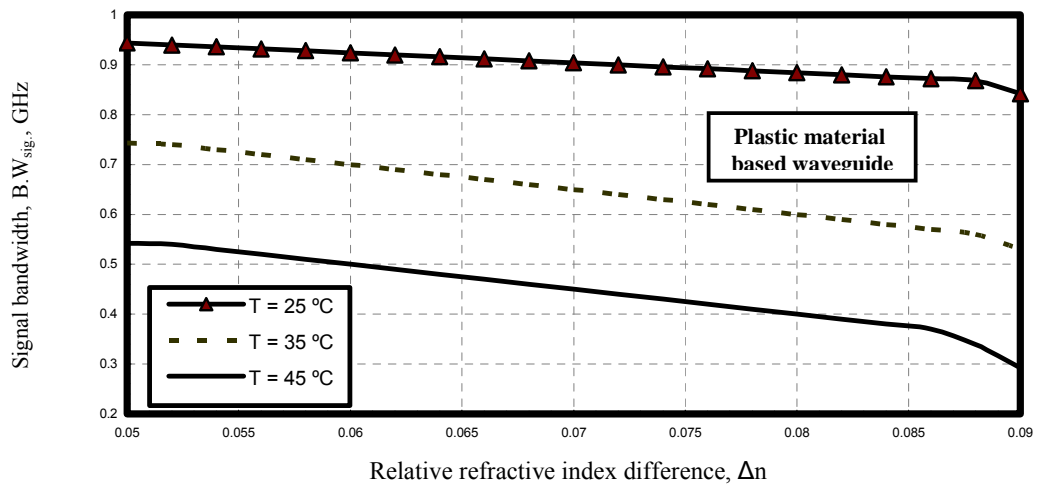
Fig. 22. Variations of signal bandwidth versus relative refractive index difference at the assumed set of parameters.
