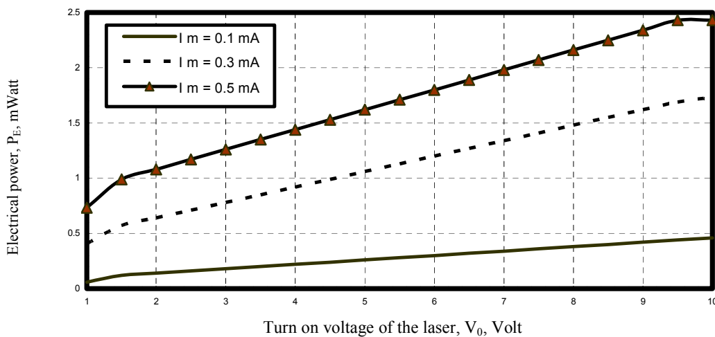
Fig. 4. Variations of electrical power against turn on voltage of the laser at the assumed set of parameters.
