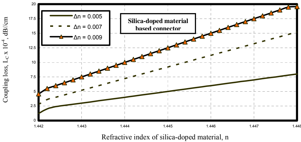
Fig. 9. Variations of coupling loss against refractive index of silica-doped material at the assumed set of parameters.
