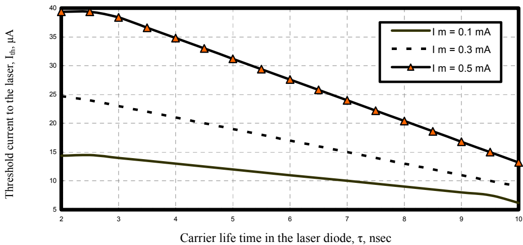
Fig. 7. Variations of threshold current to the laser against carrier life time in the laser at the assumed set of parameters.
