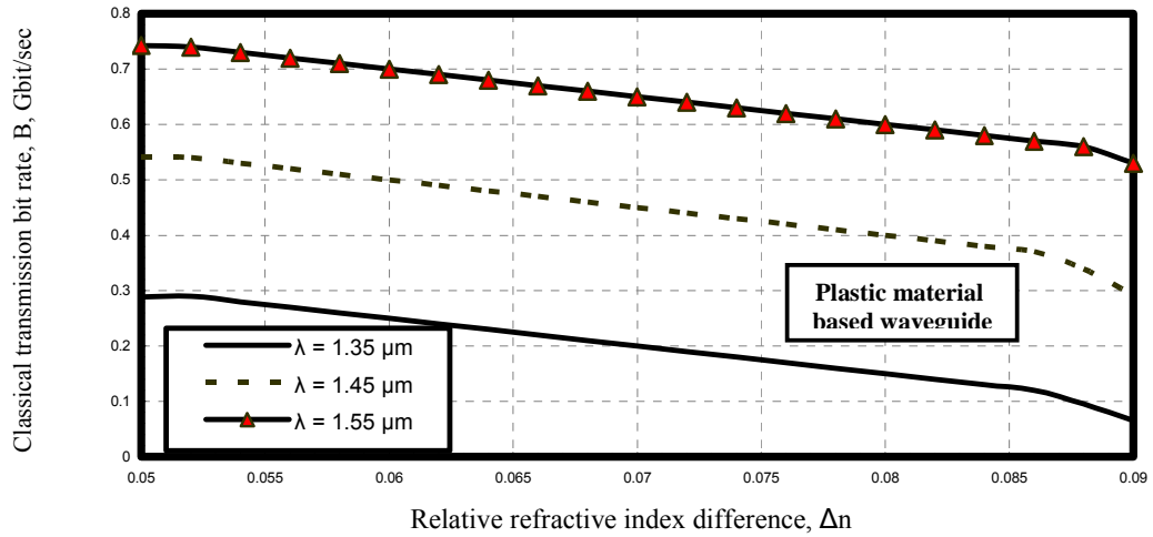
Fig. 20. Variations of classical transmission versus relative refractive index difference at the assumed set of parameters.
